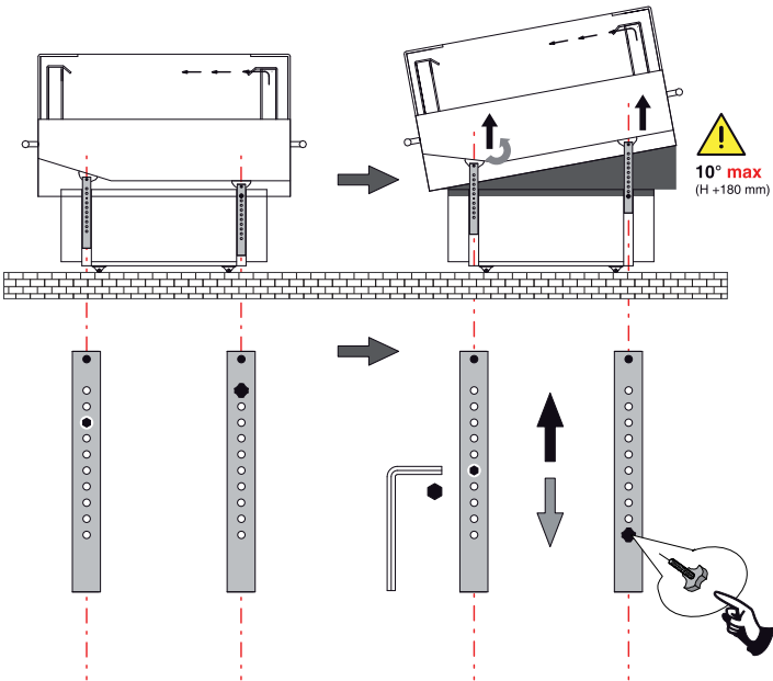
ELEVATION / INCLINATION
